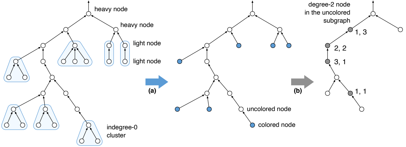
Figure 5: (a) Creating indegree-zero clusters. (b) Creating indegree-one clusters: we identify paths formed by degree-2 nodes in the subgraph induced by uncolored nodes and calculate their positions in the path both upwards and downwards.
