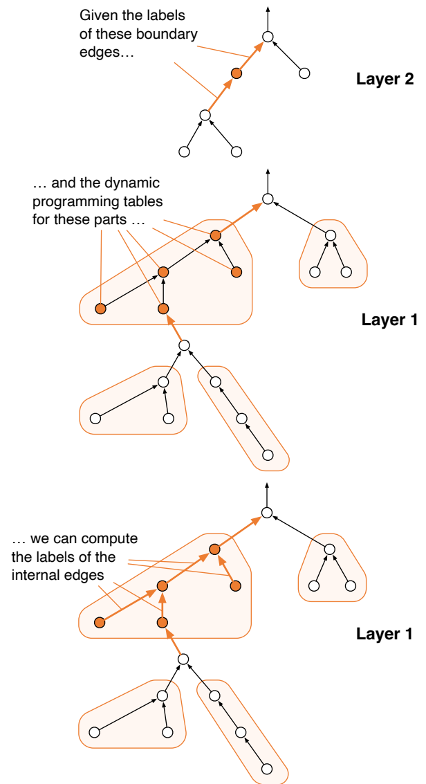
Figure 3: From top to bottom: given the solutions at the boundary edges, we assume we can compute the solution also for the internal edges.
