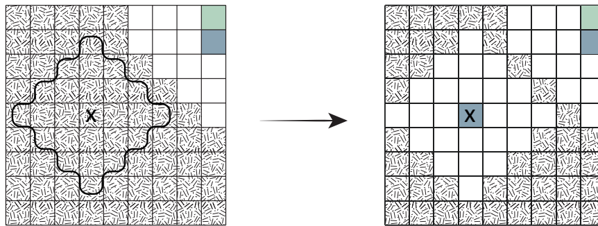
■ Figure 2 3-coloring algorithm, case 1/3. The adversary queries node x . Here node x is in the middle of an unseen region (shaded). The algorithm creates a new group (white) and fixes the color of node x arbitrarily.
